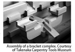
Assembly of a bracket complex. Courtesy of Takenaka Carpentry Tools Museum
